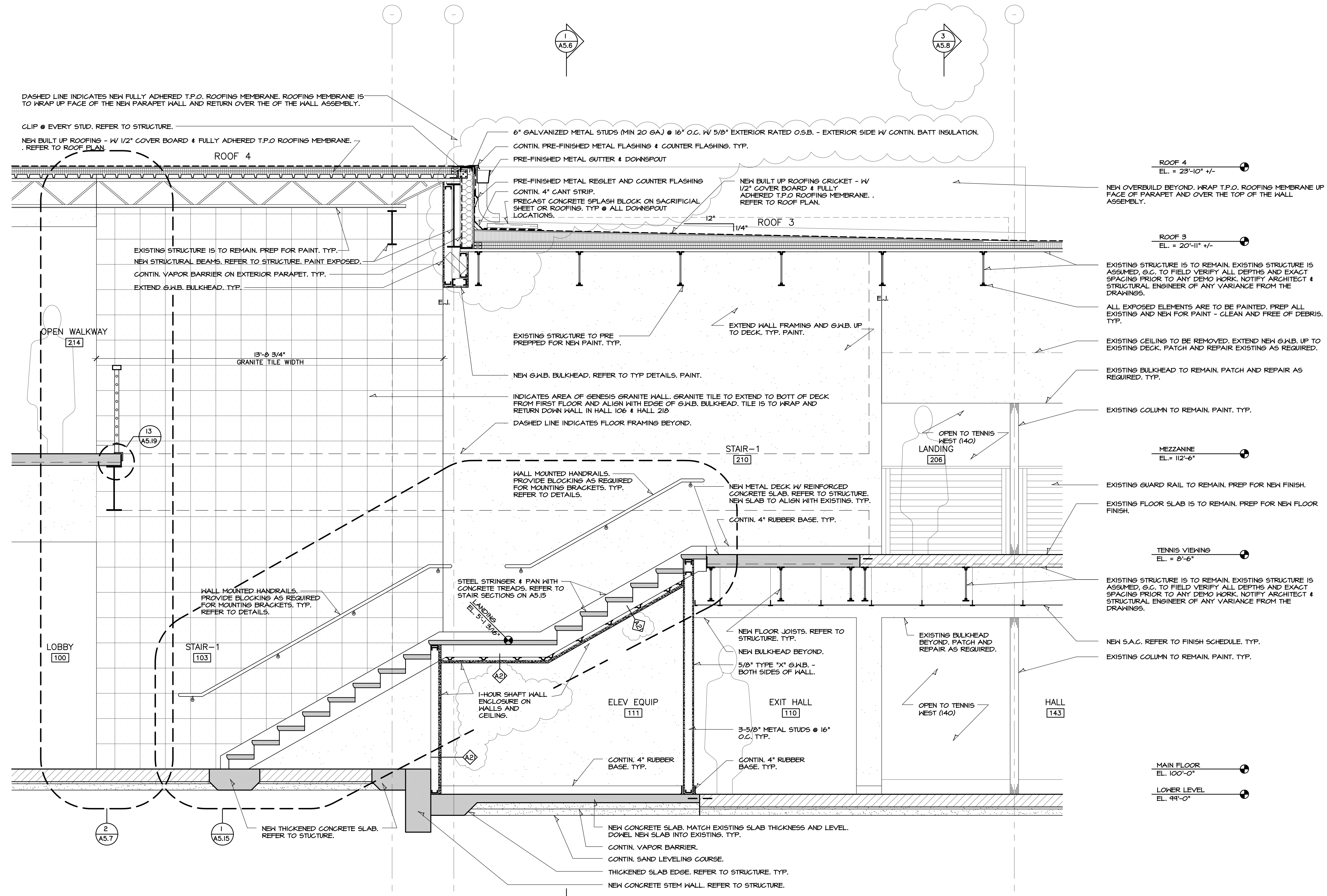
1 WALL SECTION SCALE 1/2" = 1'-0"
