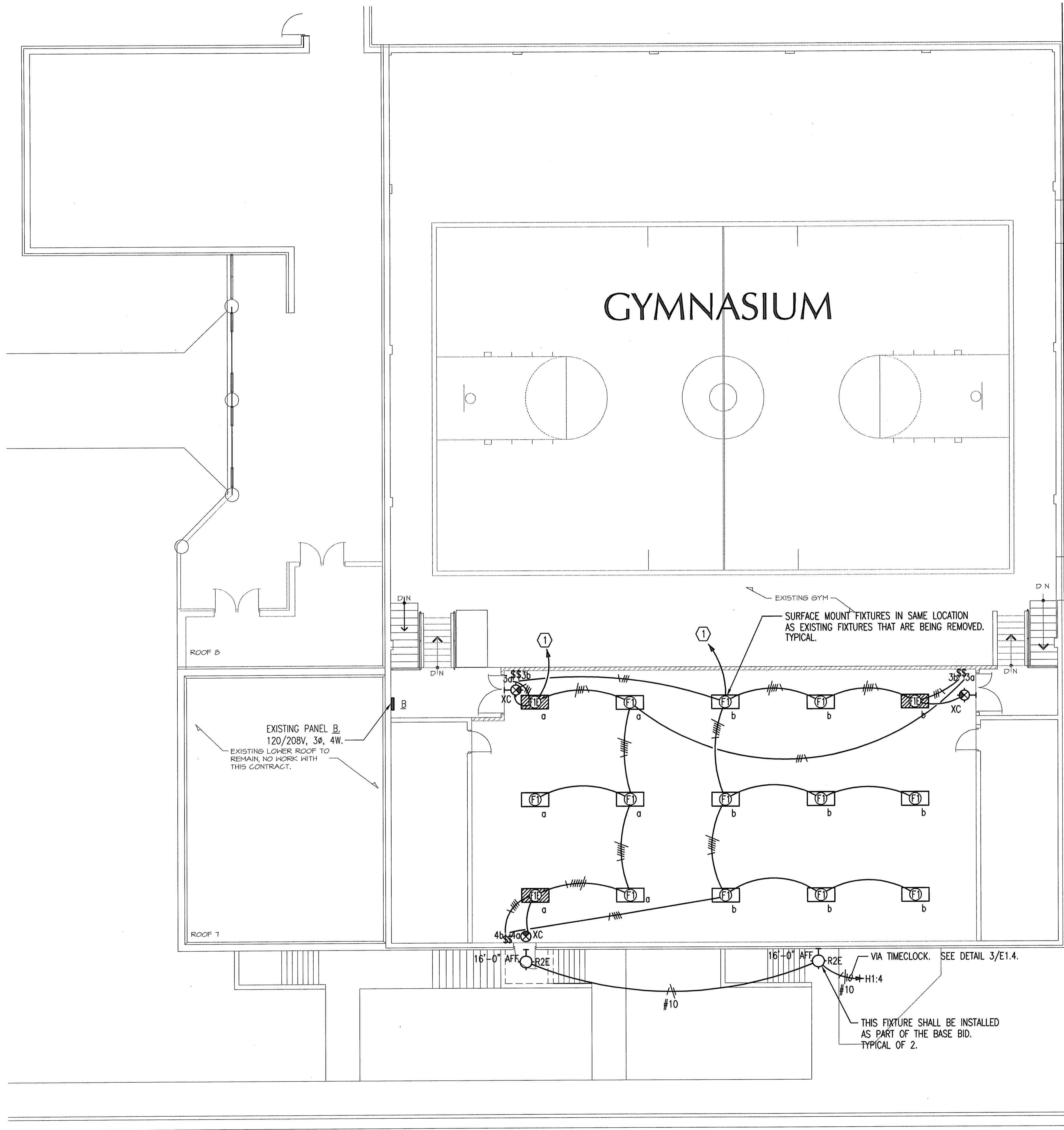
ELECTRICAL LIGHTING PLAN - ALTERNATE #4 1/8" = 1'-0"
