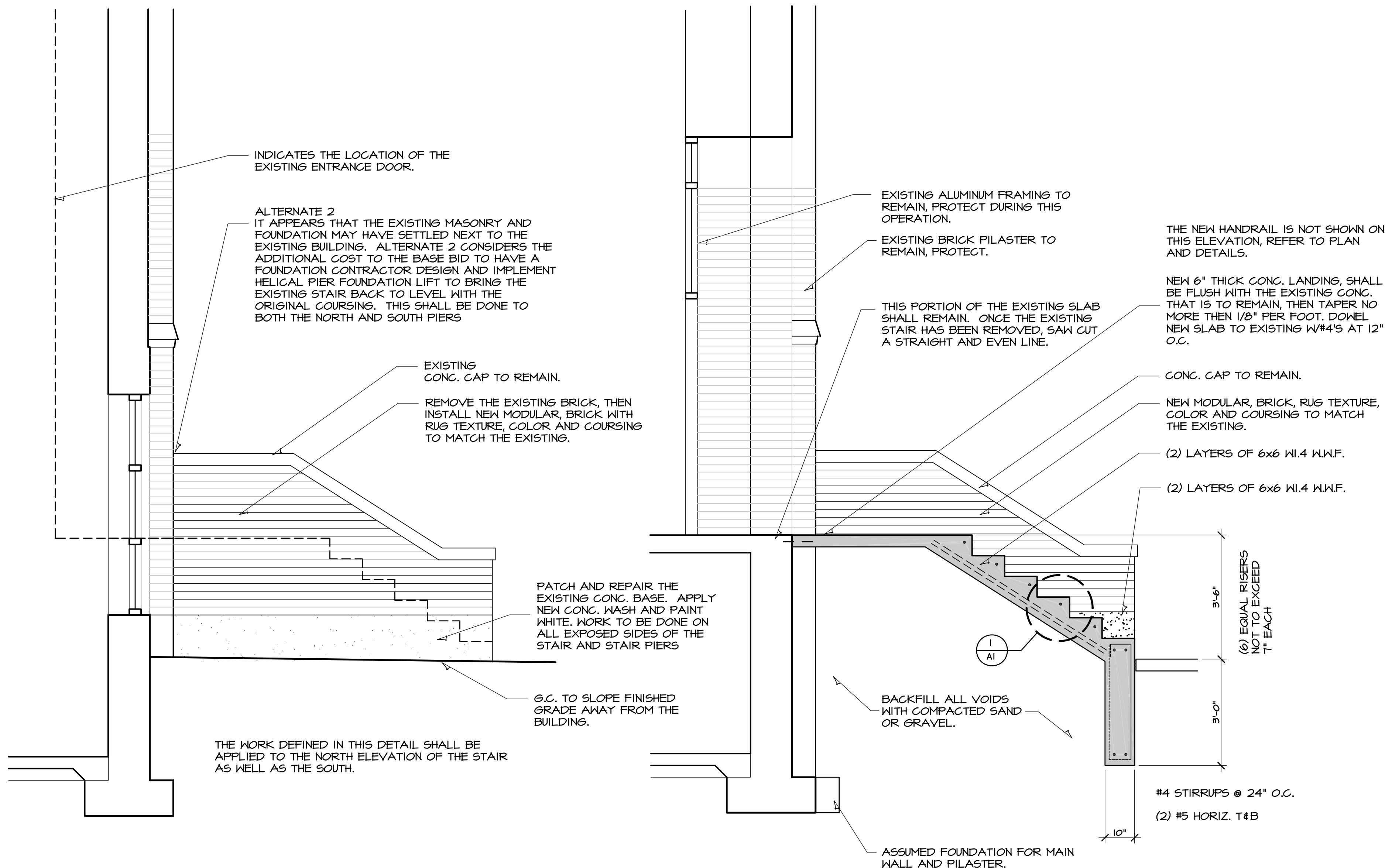
1 SOUTH ELEVATION SCALE 1/2" = 1'-0"
