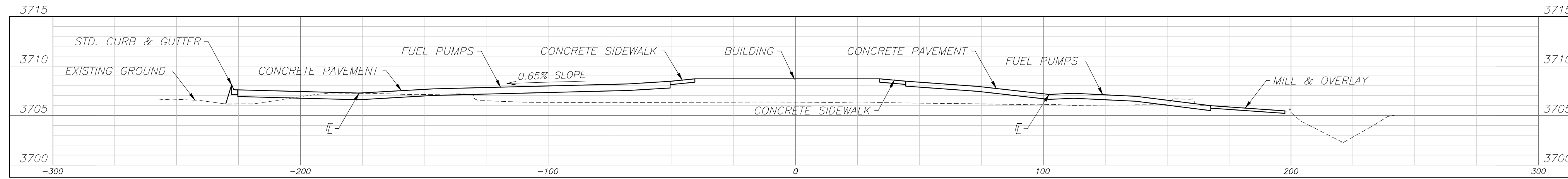
SECTION C-C
