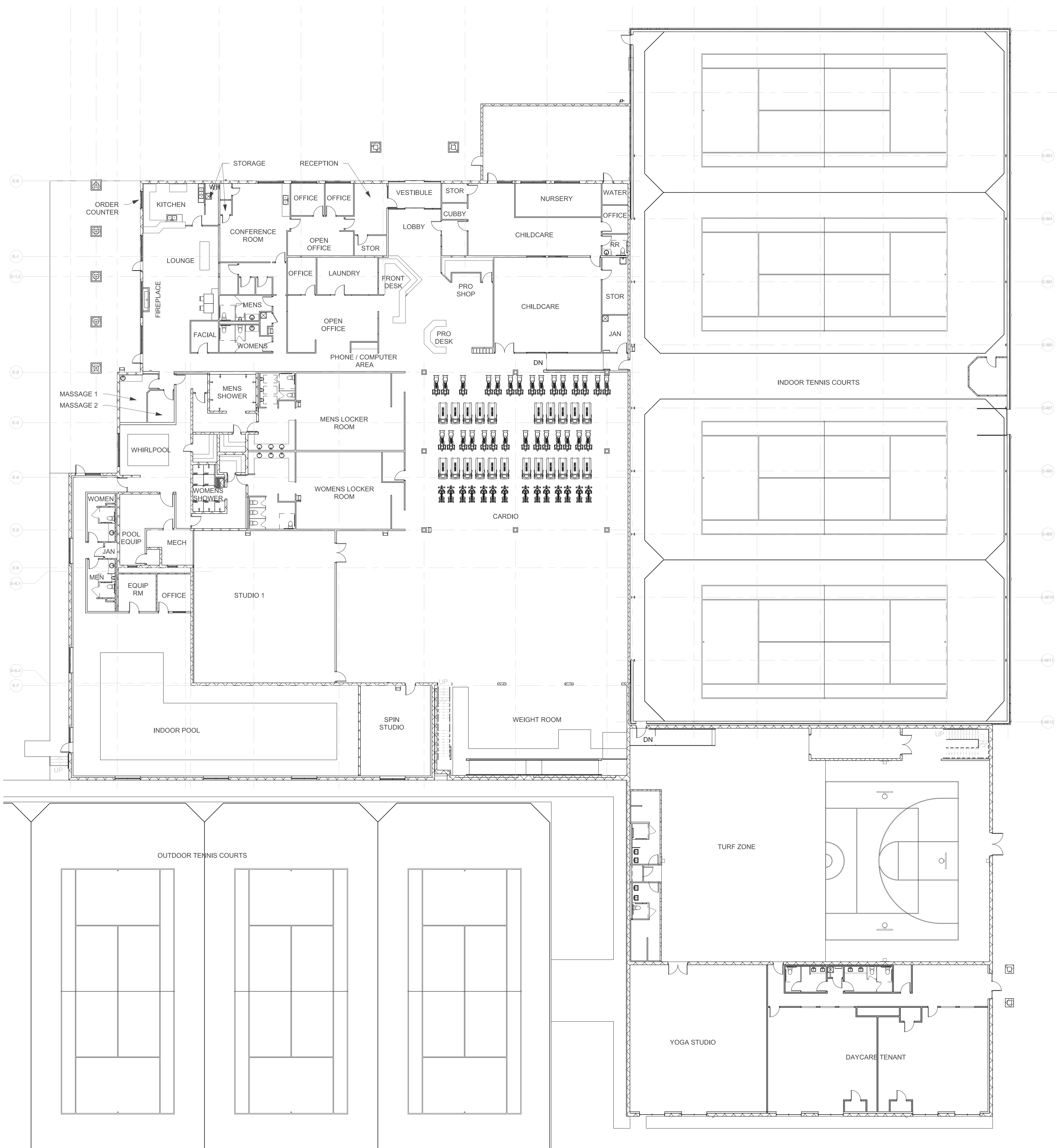
A EXISTING OVERALL FIRST FLOOR PLAN SCALE: 1/16" = 1'-0"
